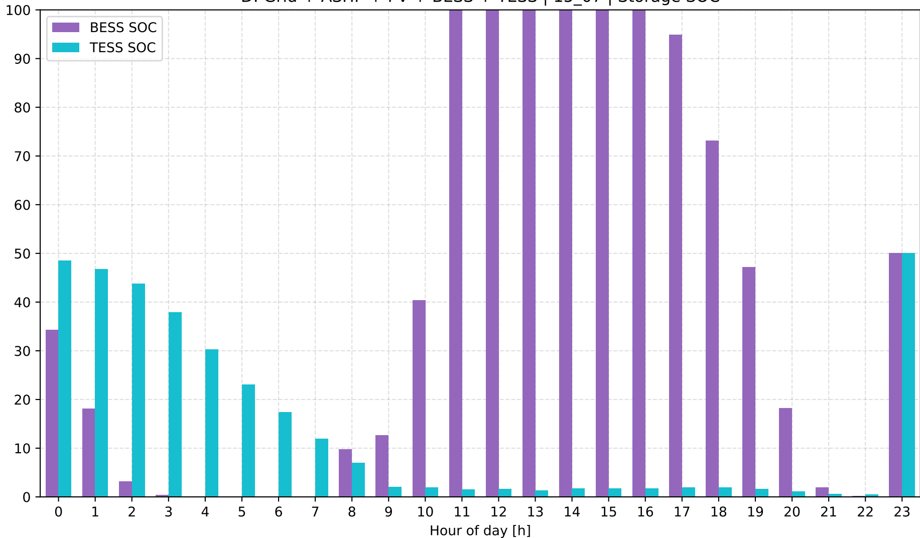
D: Grid + ASHP + PV + BESS + TESS | 15_07 | Storage SOC
