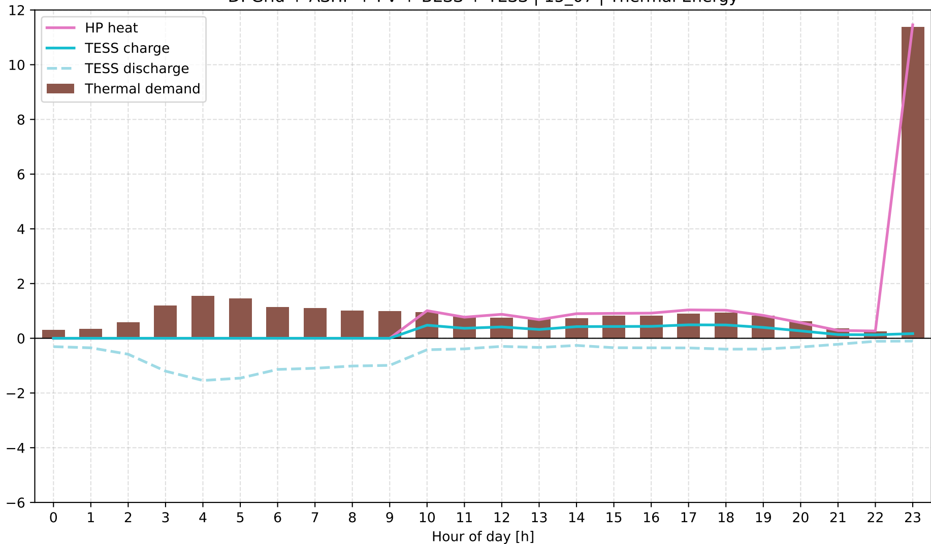
D: Grid + ASHP + PV + BESS + TESS | 15_07 | Thermal Energy
