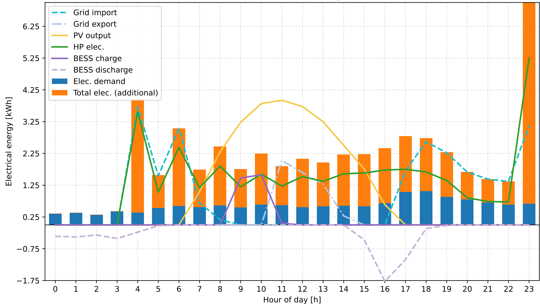
D: Grid + ASHP + PV + BESS + TESS | 15_10 | Electrical Energy
