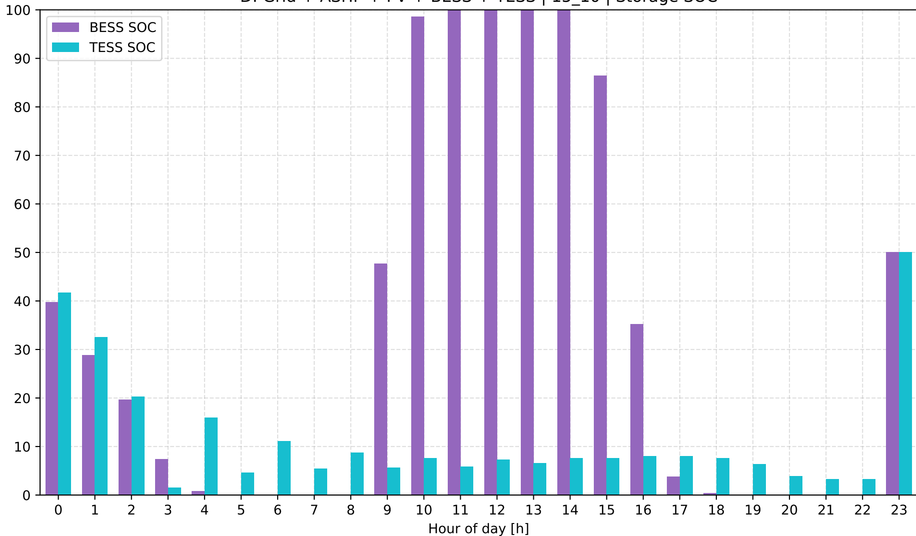
D: Grid + ASHP + PV + BESS + TESS | 15_10 | Storage SOC
