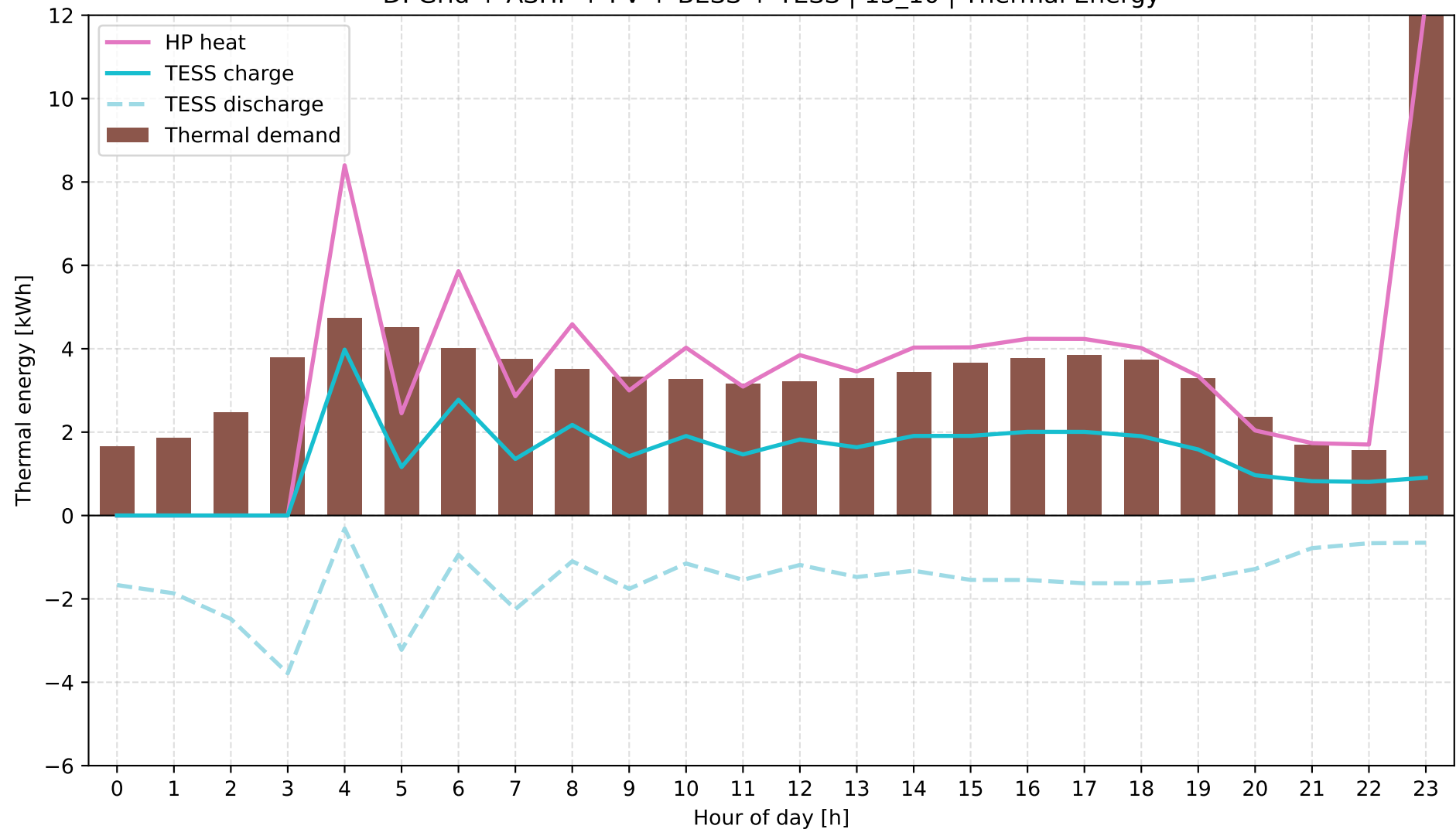
D: Grid + ASHP + PV + BESS + TESS | 15_10 | Thermal Energy
