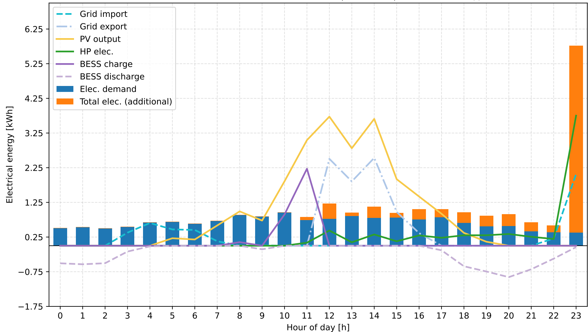
D: Grid + ASHP + PV + BESS + TESS | Summer | Electrical Energy
