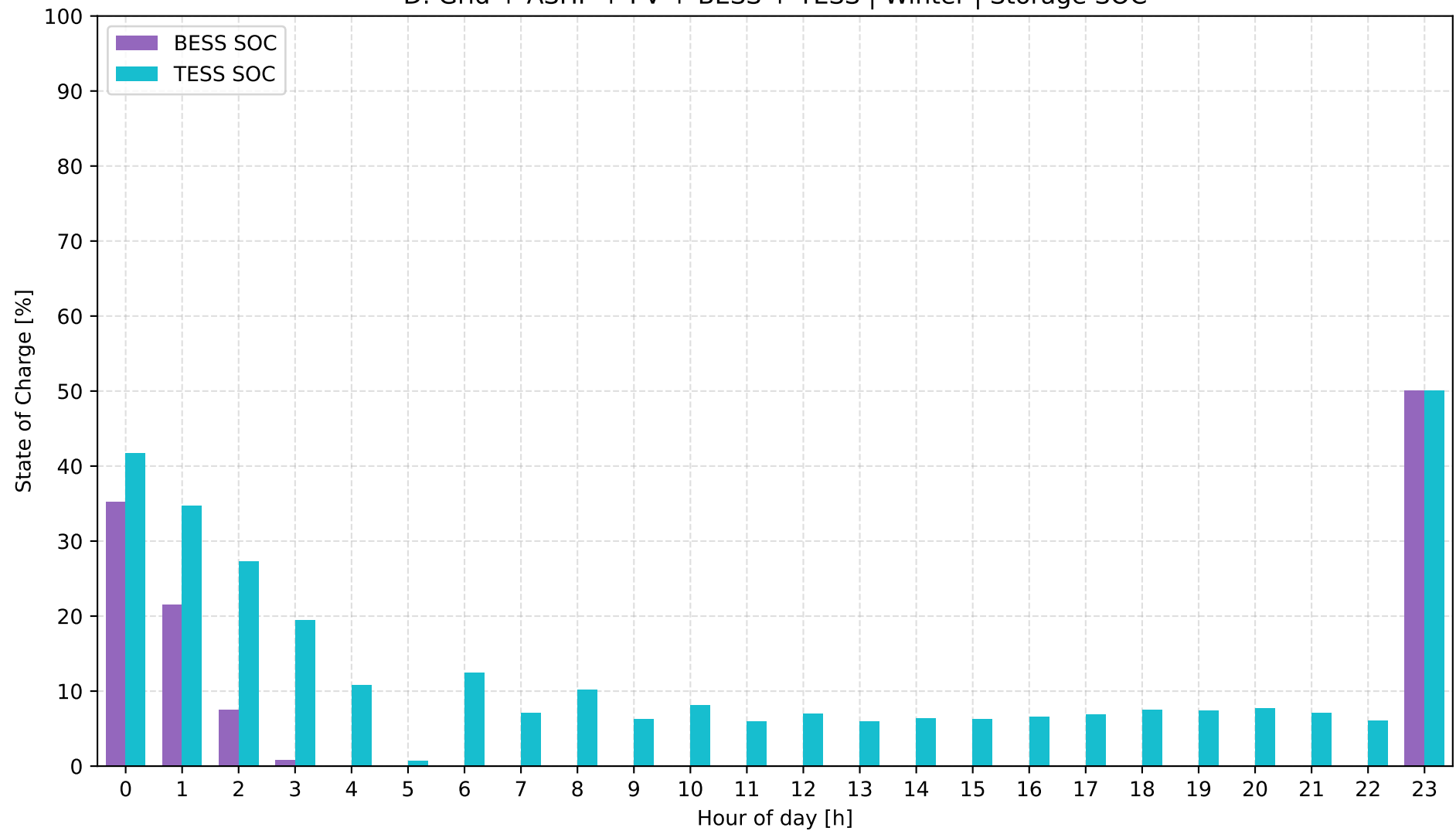
D: Grid + ASHP + PV + BESS + TESS | Winter | Storage SOC
