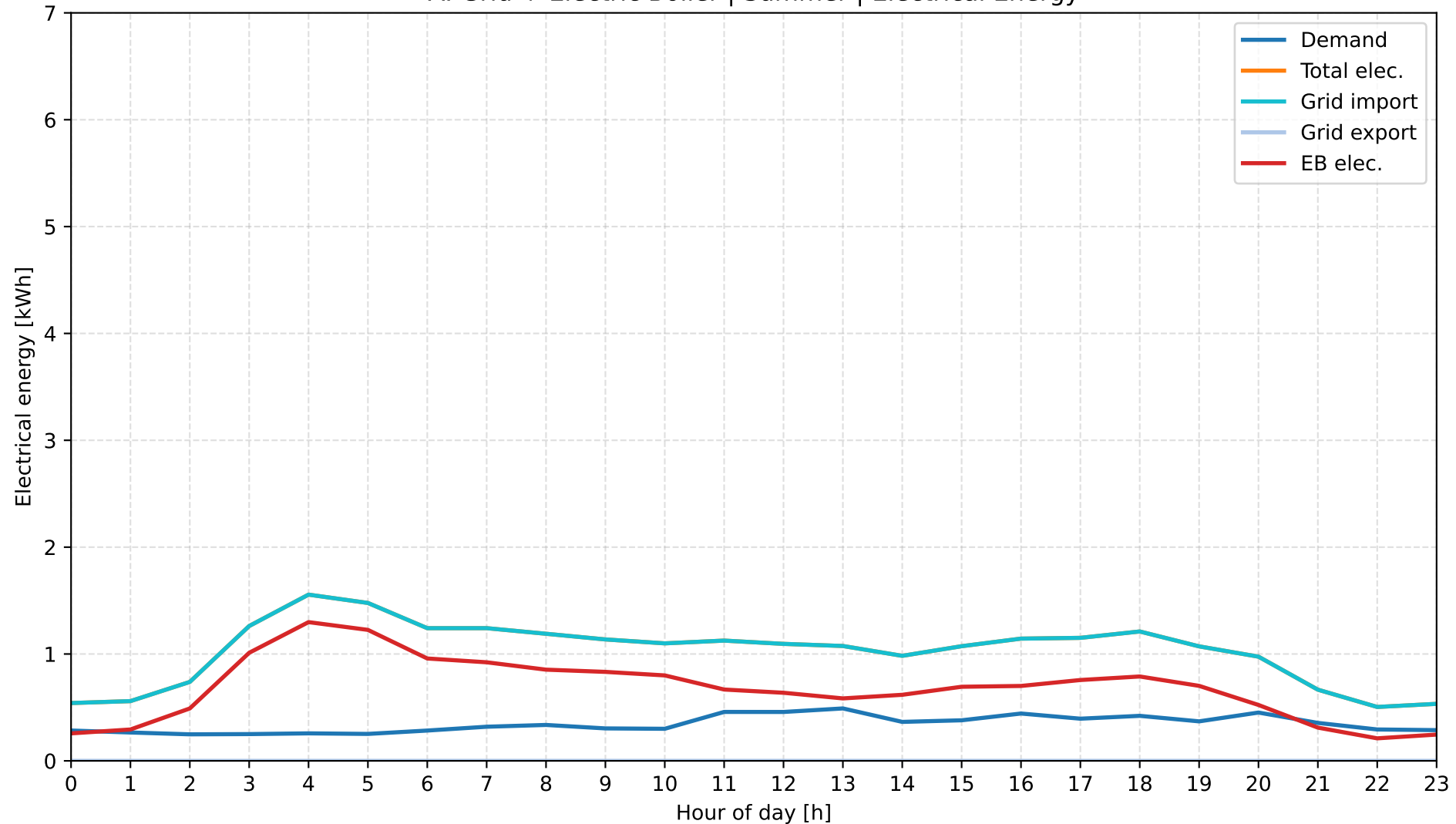
A: Grid + Electric Boiler | Summer | Electrical Energy
