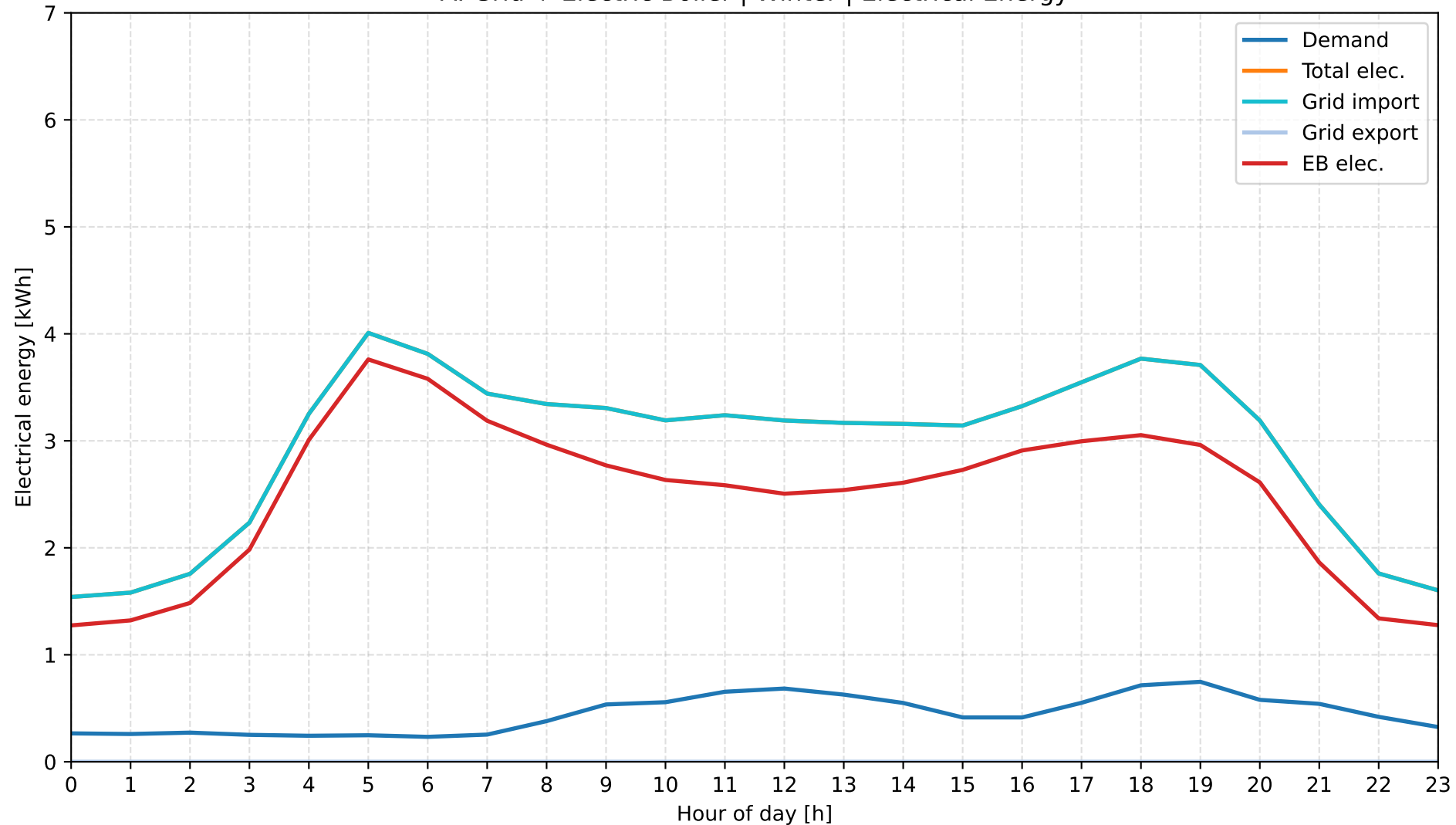
A: Grid + Electric Boiler | Winter | Electrical Energy
