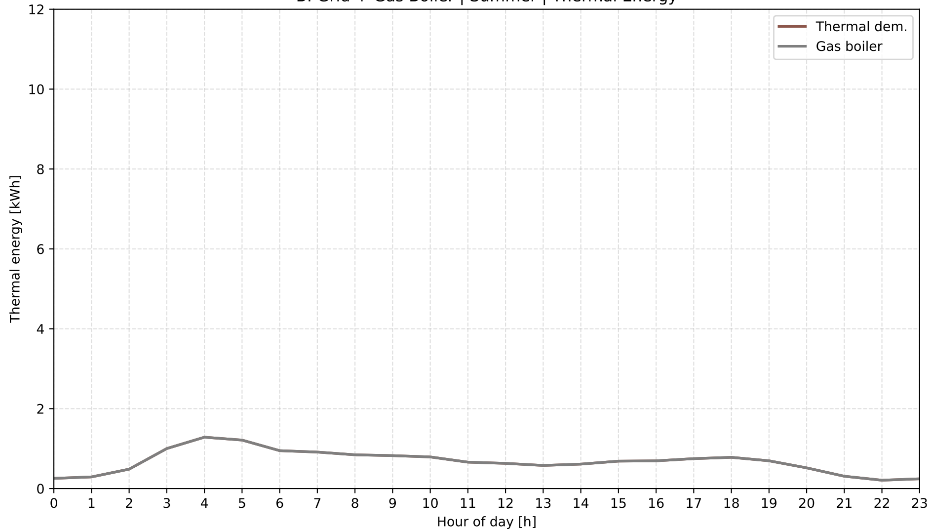
B: Grid + Gas Boiler | Summer | Thermal Energy
