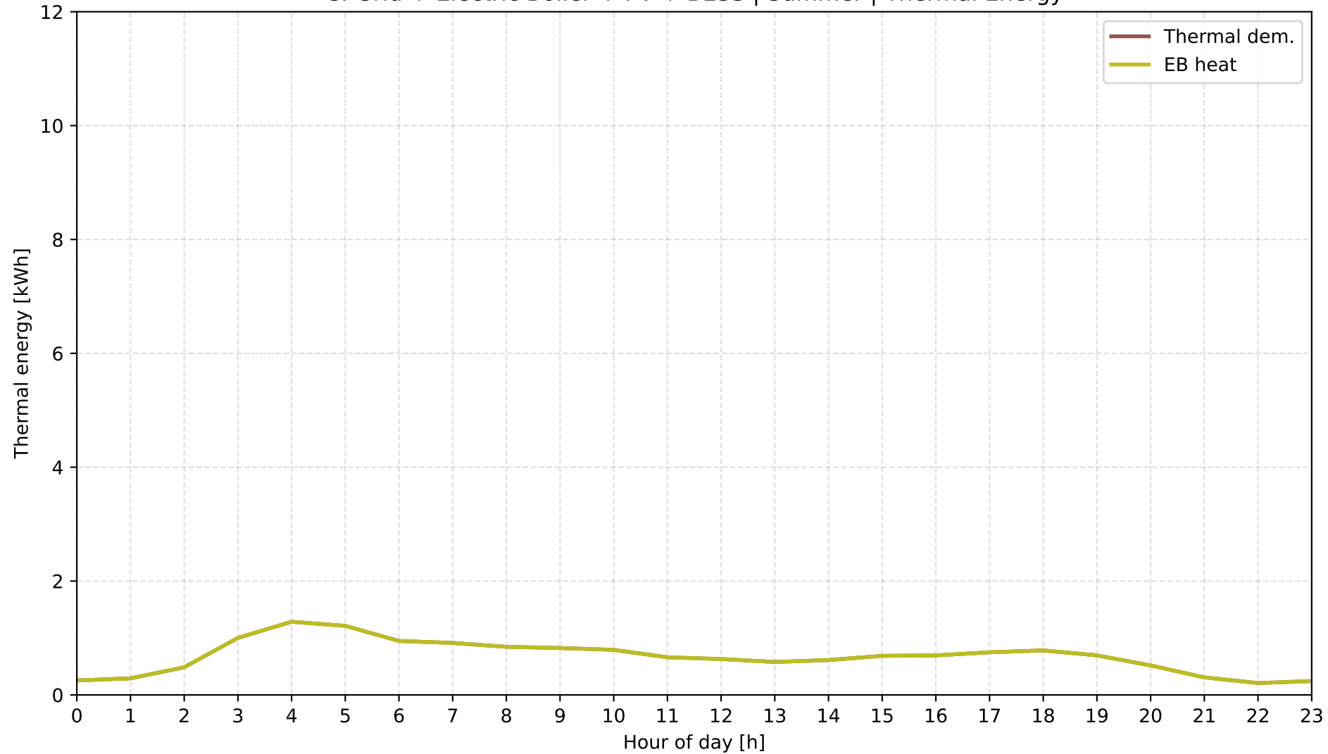
C: Grid + Electric Boiler + PV + BESS | Summer | Thermal Energy
