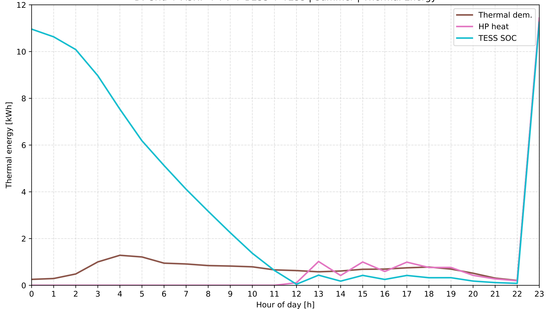
D: Grid + ASHP + PV + BESS + TESS | Summer | Thermal Energy
