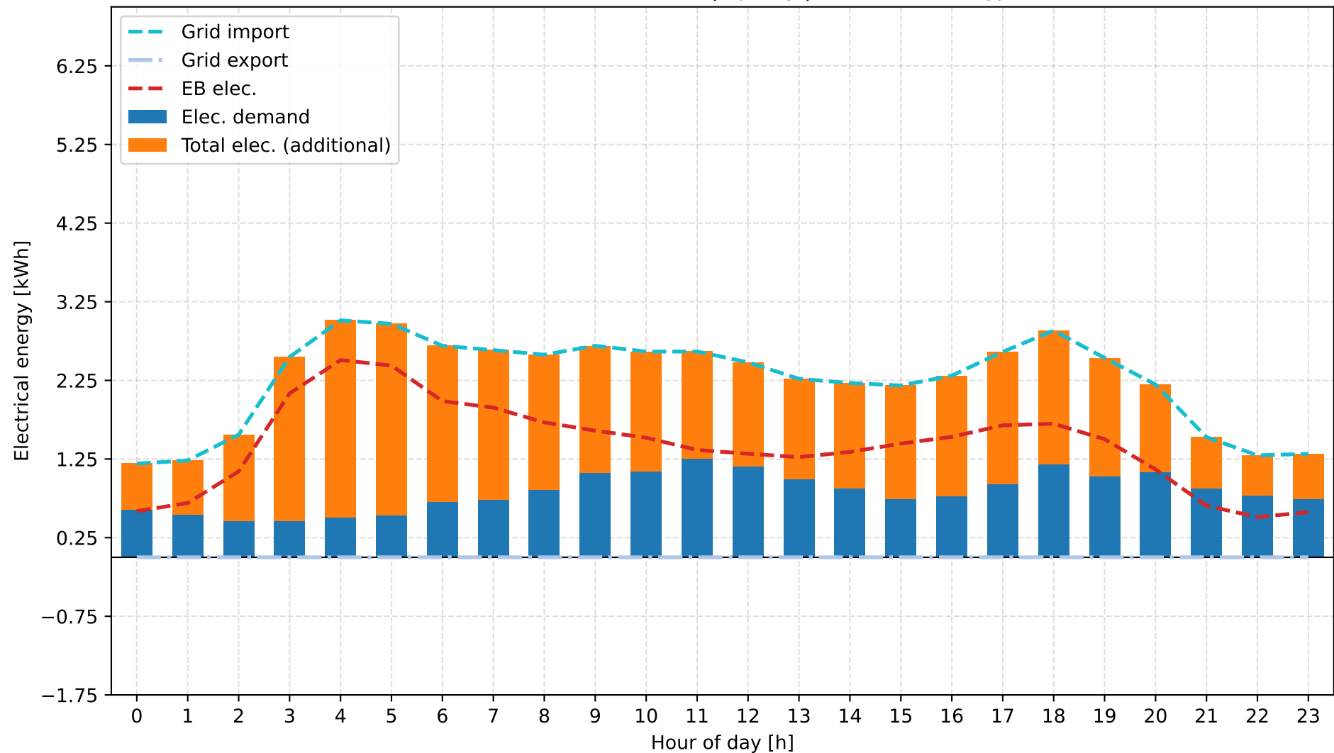
B: Grid + Electric Boiler | spring | Electrical Energy
