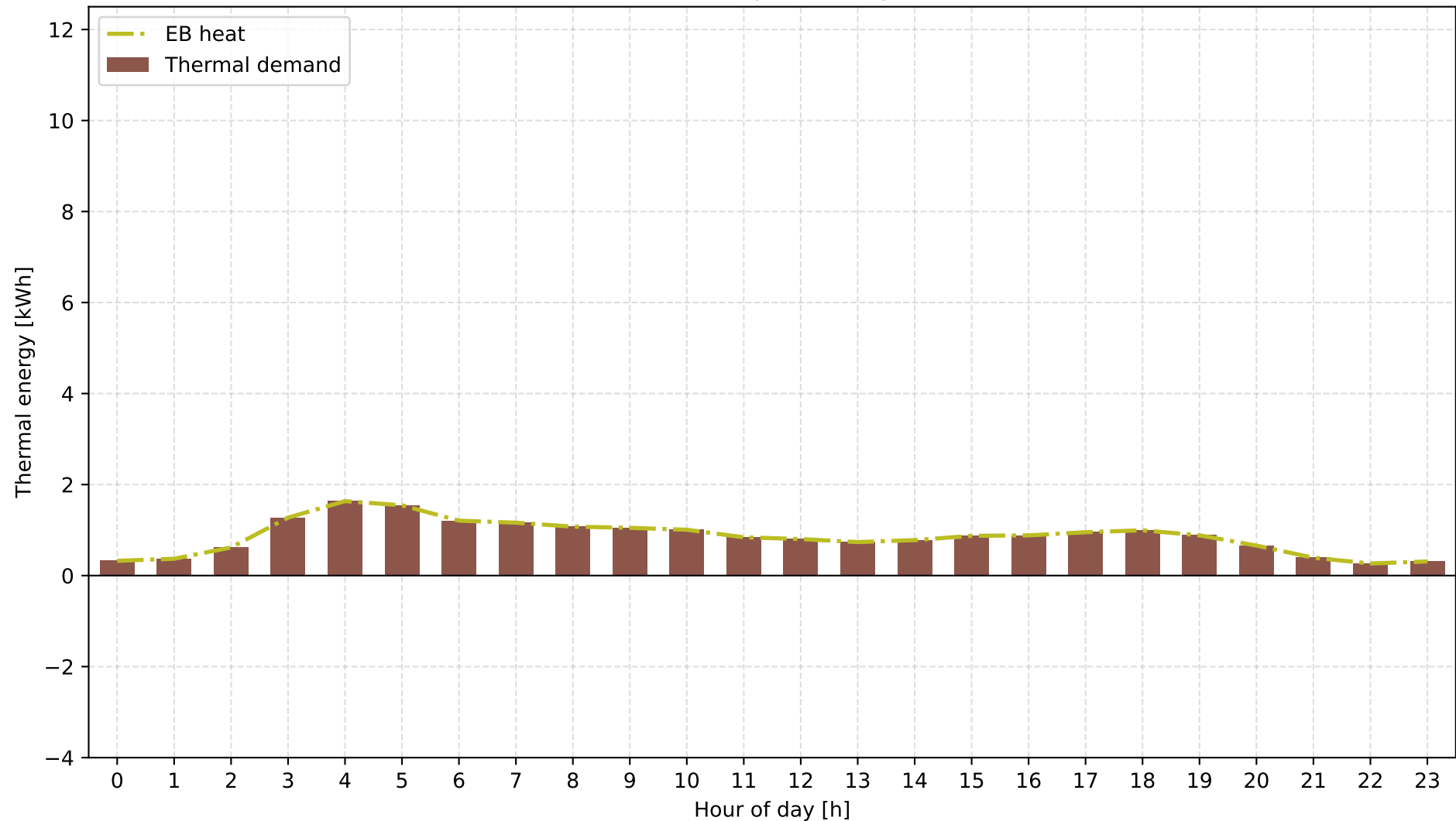
B: Grid + Electric Boiler | summer | Thermal Energy
