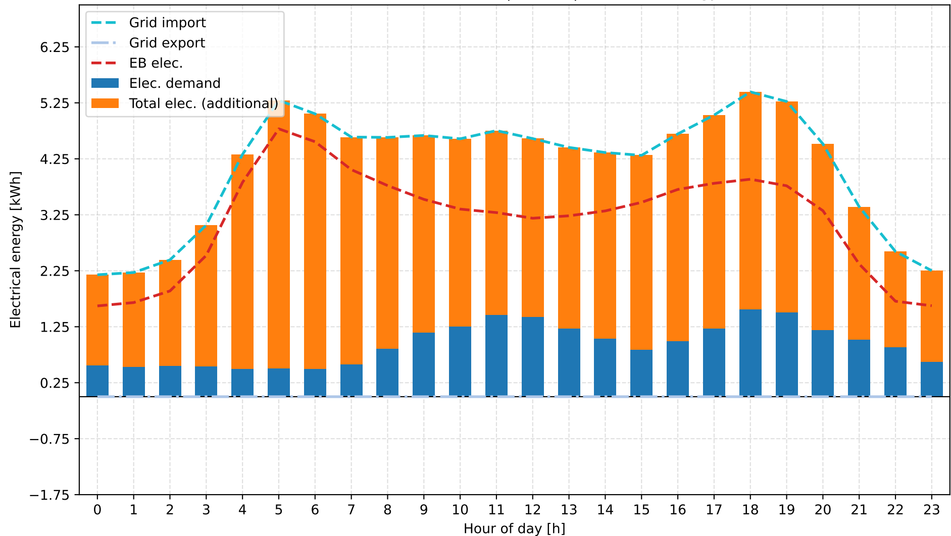
B: Grid + Electric Boiler | winter | Electrical Energy
