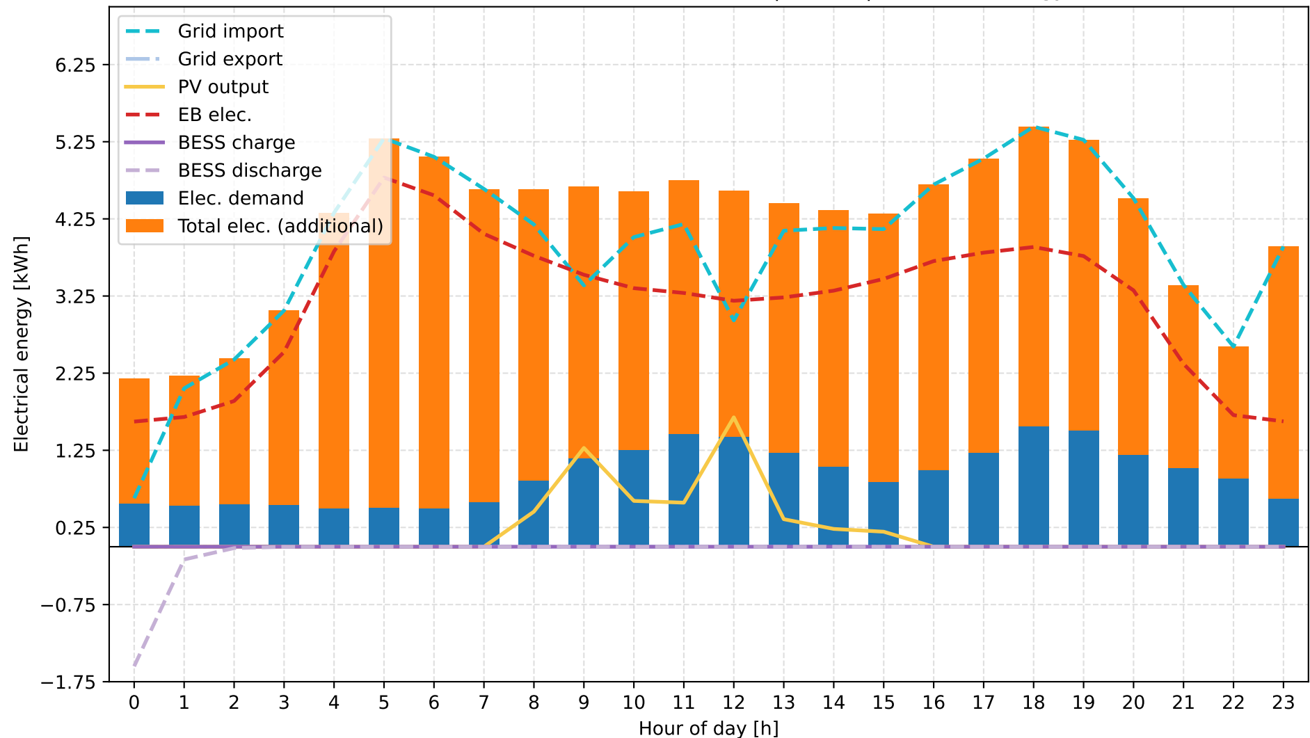
C: Grid + Electric Boiler + PV + BESS | winter | Electrical Energy
