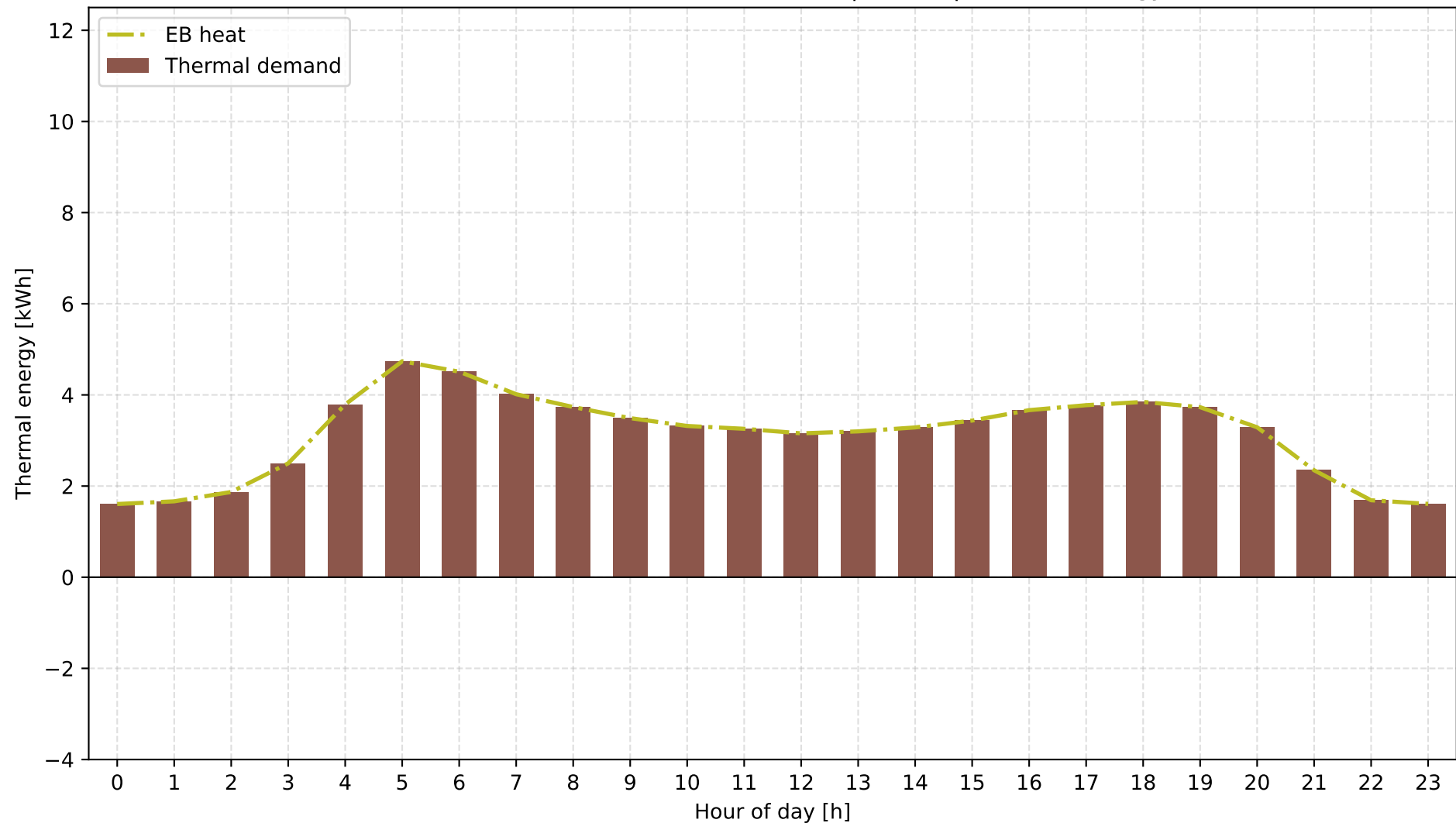
C: Grid + Electric Boiler + PV + BESS | winter | Thermal Energy
