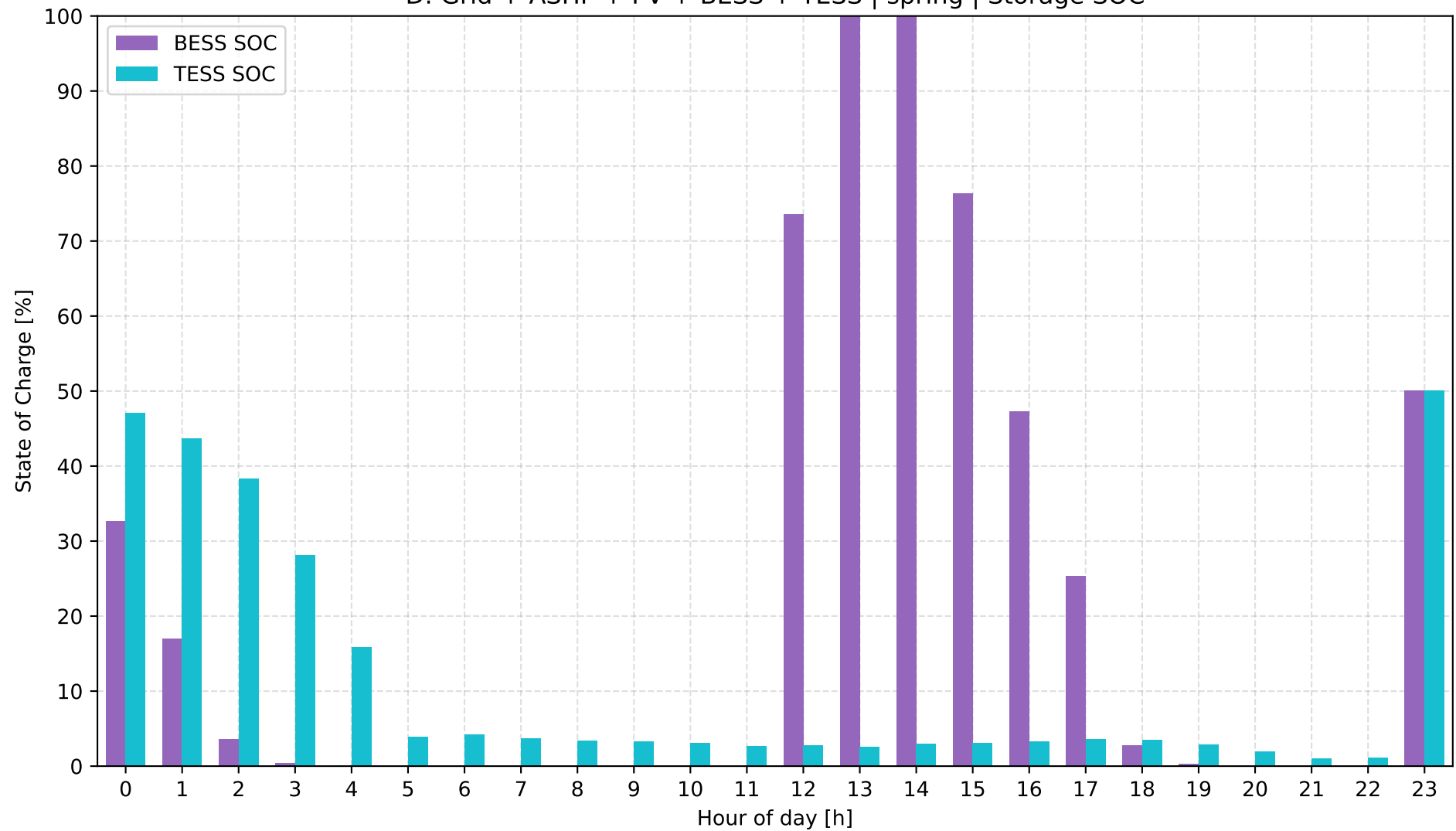
D: Grid + ASHP + PV + BESS + TESS | spring | Storage SOC
