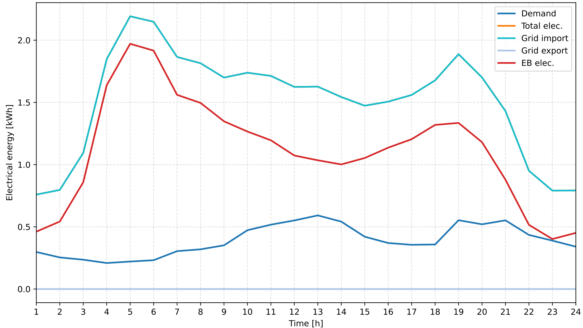
Spring — Electrical Energy
