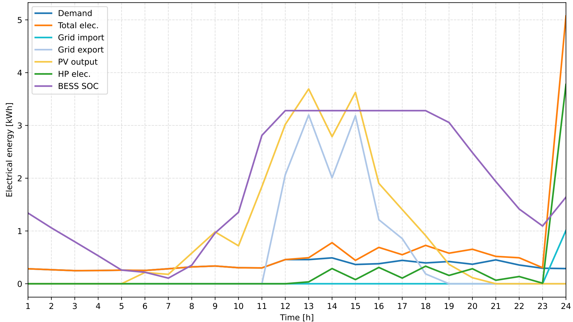
Summer — Electrical Energy
