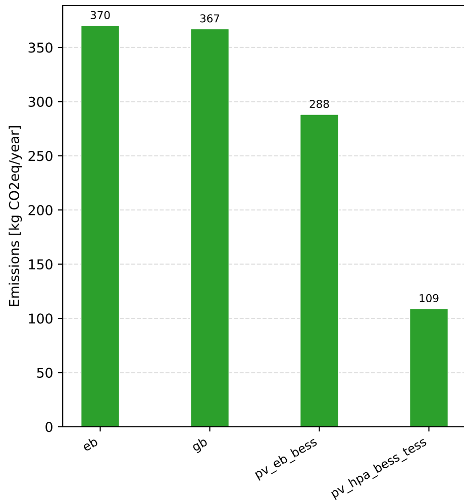
Annual Total Emissions
