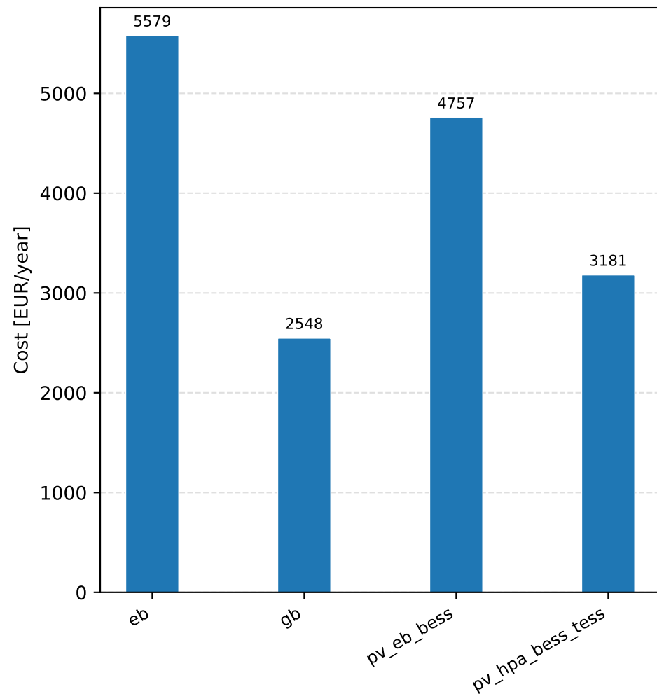
Annual Total Cost
