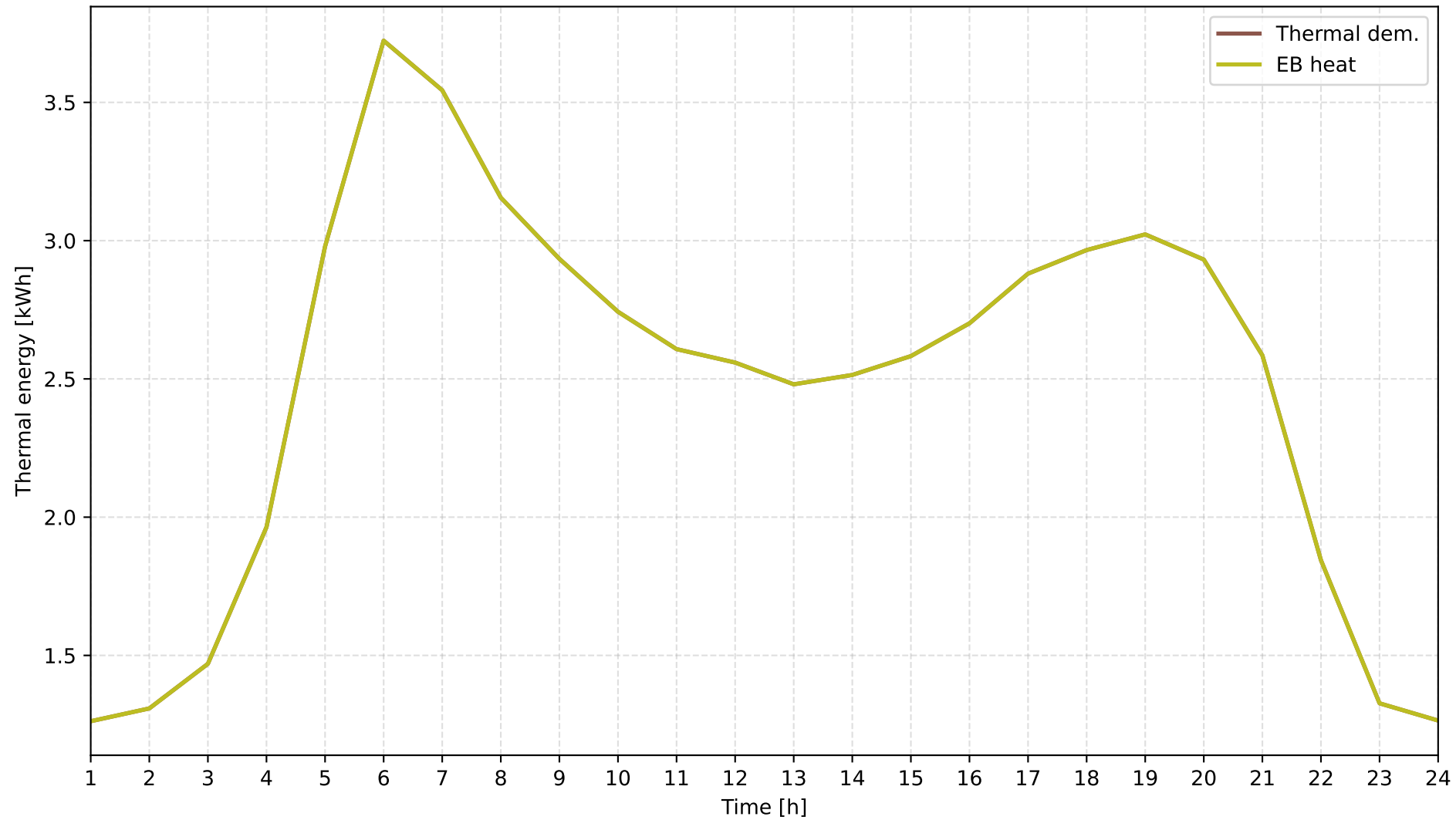
Winter — Thermal Energy
