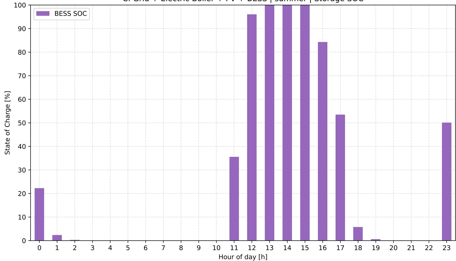
C: Grid + Electric Boiler + PV + BESS | summer | Storage SOC
