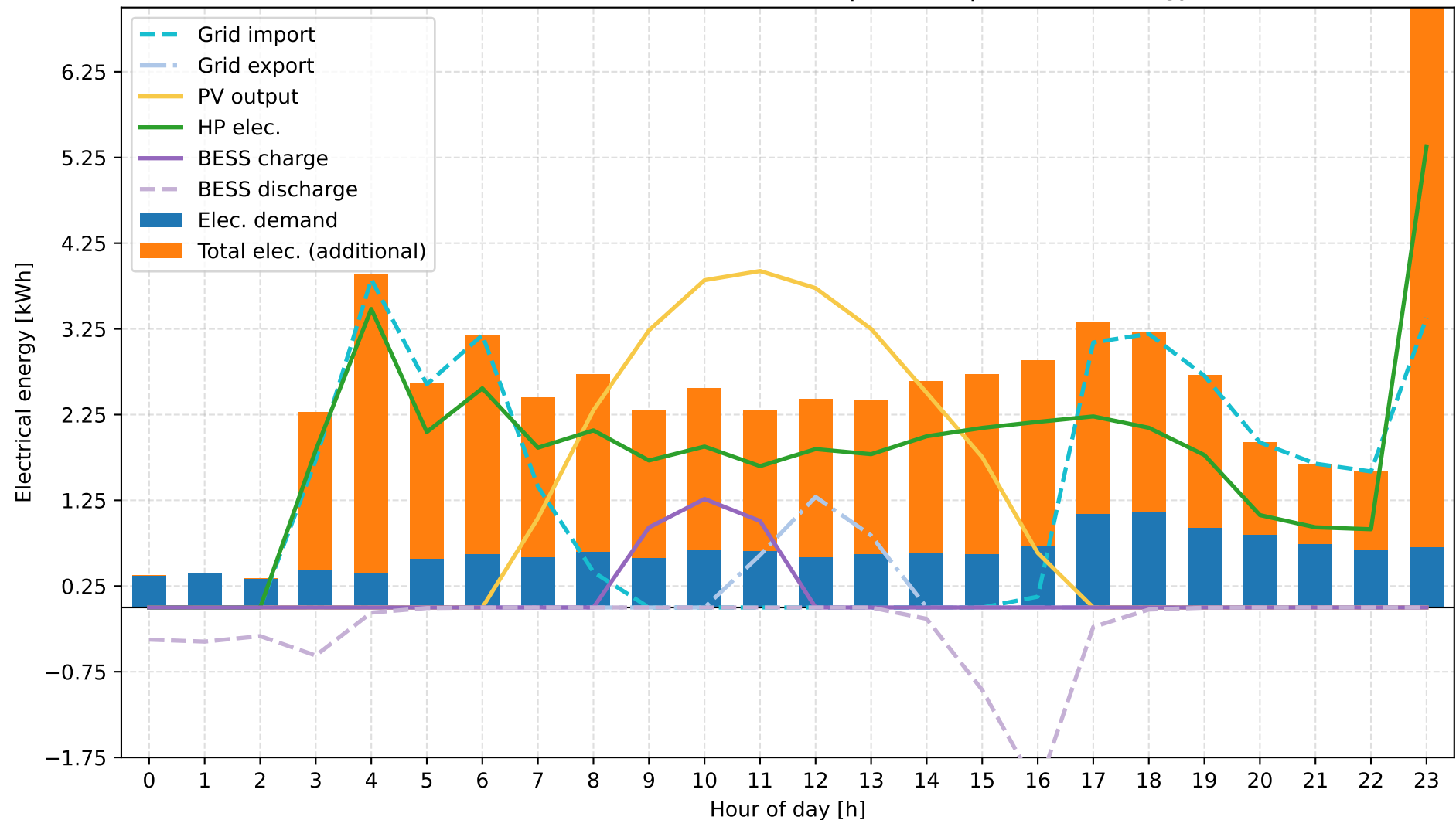
D: Grid + ASHP + PV + BESS + TESS | autumn | Electrical Energy
