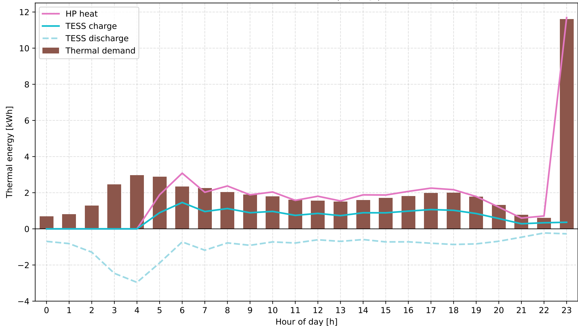
D: Grid + ASHP + PV + BESS + TESS | spring | Thermal Energy
