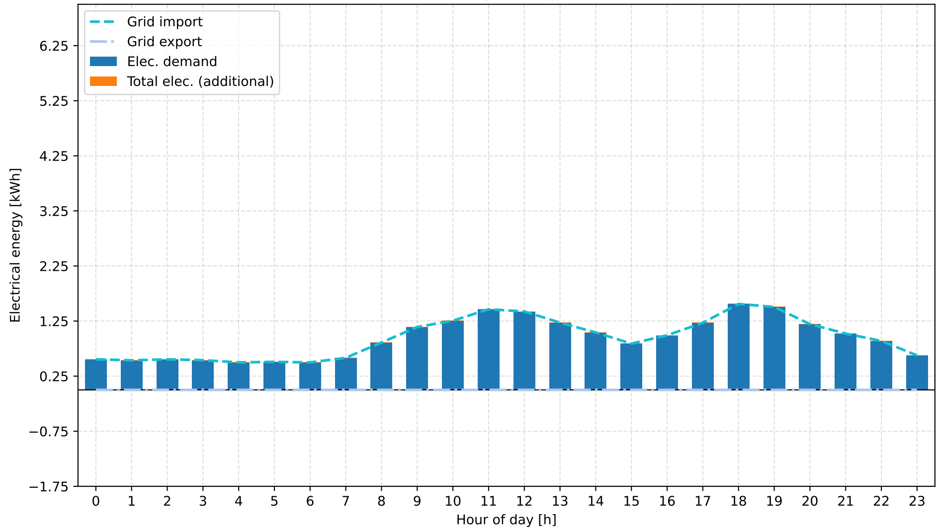
A: Grid + Gas Boiler | winter | Electrical Energy
