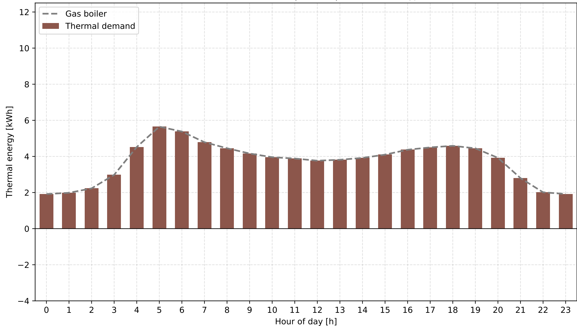
A: Grid + Gas Boiler | winter | Thermal Energy
