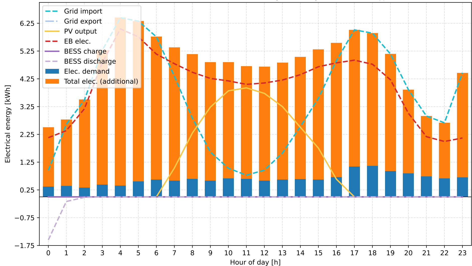
C: Grid + Electric Boiler + PV + BESS | autumn | Electrical Energy
