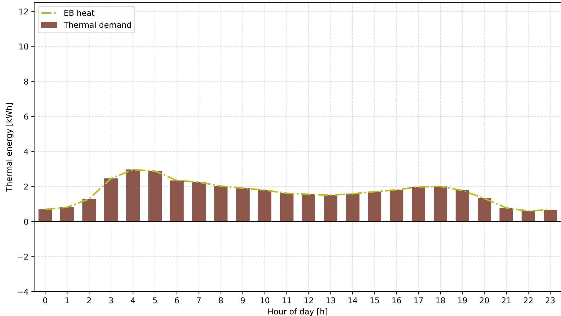
C: Grid + Electric Boiler + PV + BESS | spring | Thermal Energy
