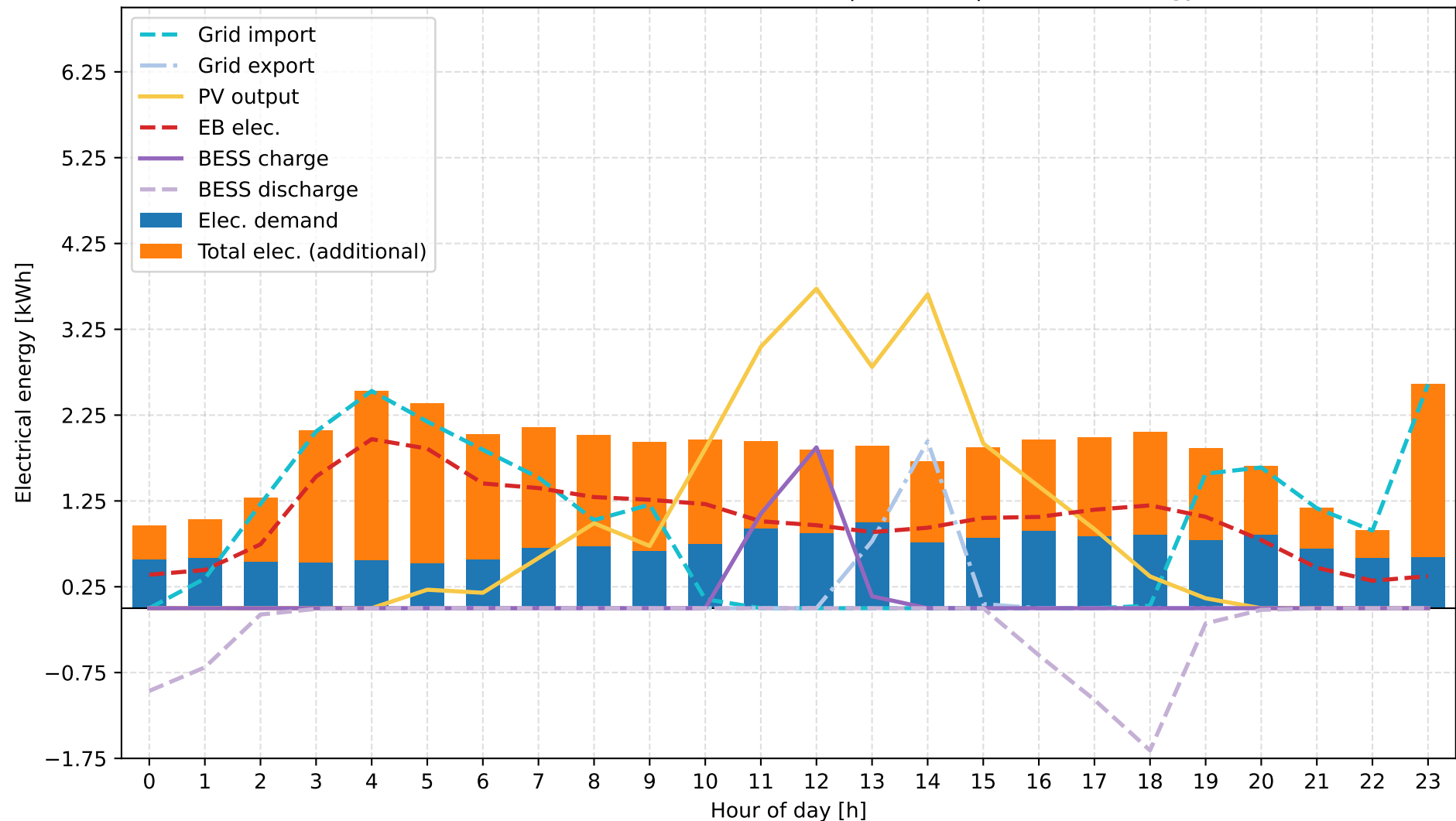
C: Grid + Electric Boiler + PV + BESS | summer | Electrical Energy
