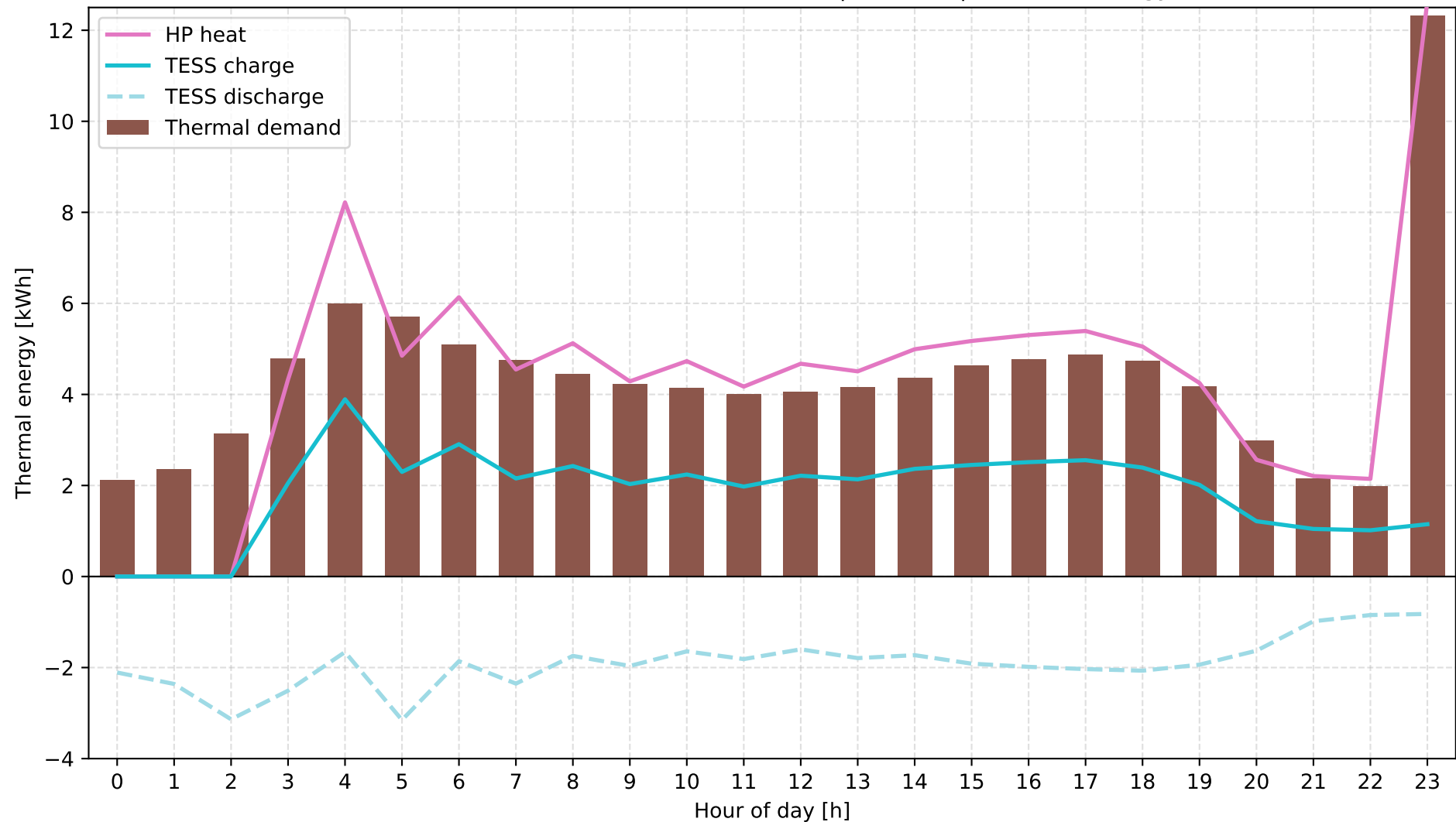
D: Grid + ASHP + PV + BESS + TESS | autumn | Thermal Energy
