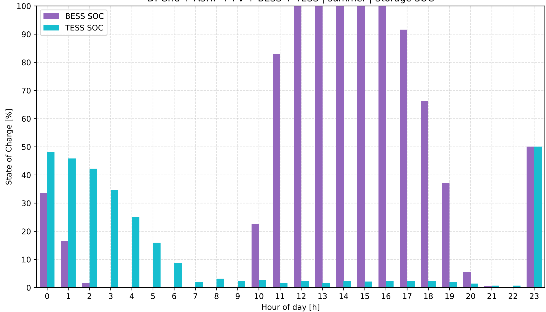
D: Grid + ASHP + PV + BESS + TESS | summer | Storage SOC
