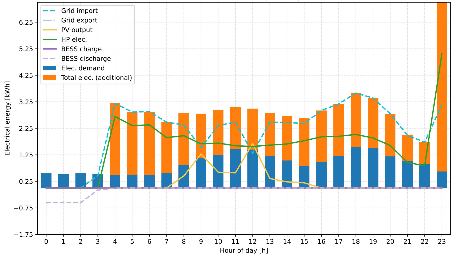
D: Grid + ASHP + PV + BESS + TESS | winter | Electrical Energy
