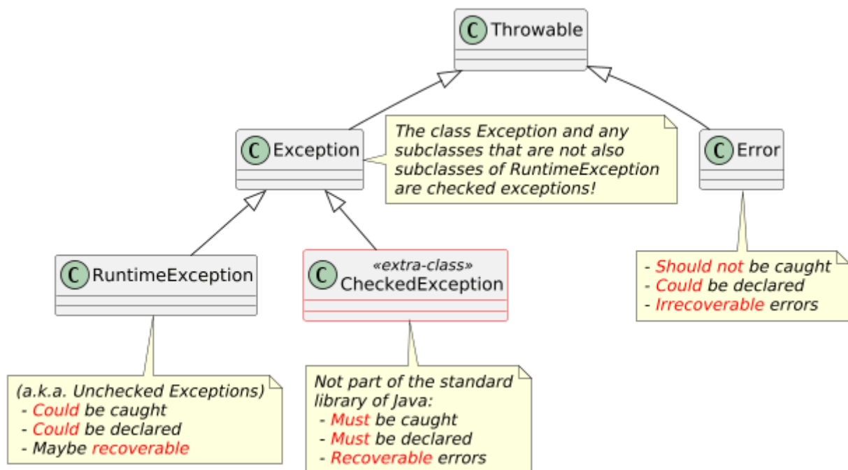
Figure 1. Exceptions Hierarchie
