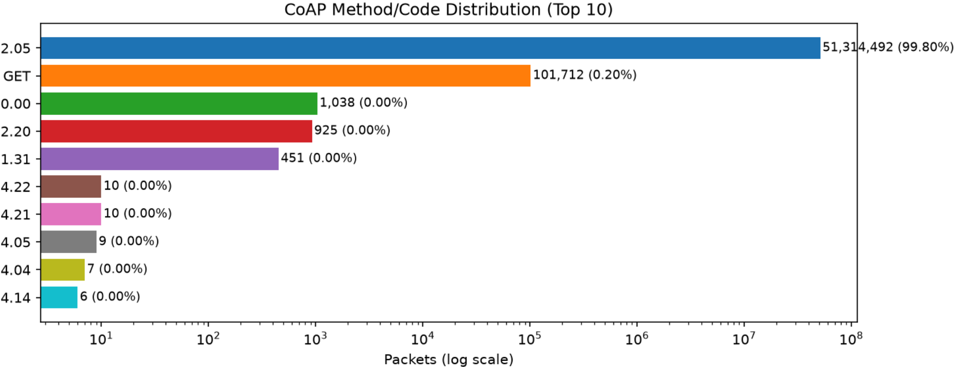
Figure 10: Share of CoAP Codes
