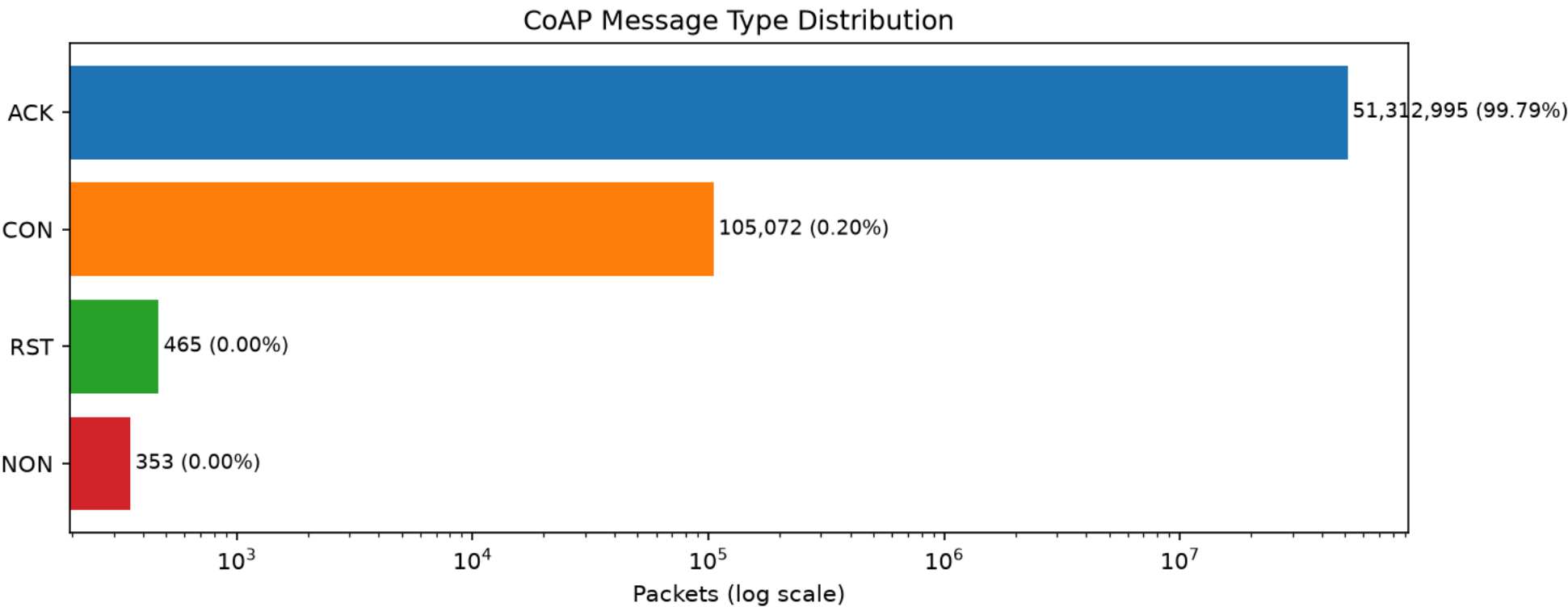
Figure 9: Share of CoAP Message Types
