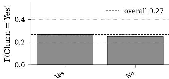
PhoneService
