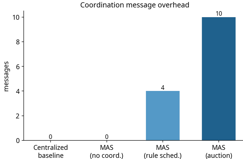
Figure 7.3: Coordination message overhead per 60 s scenario run.
