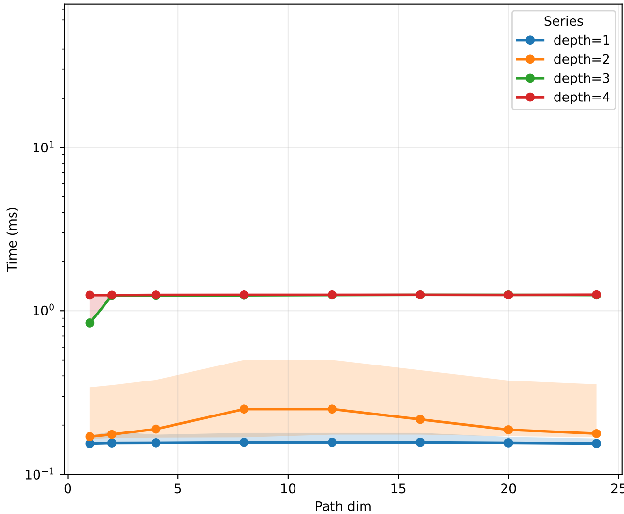
Signature Compute Time (shuffle)
