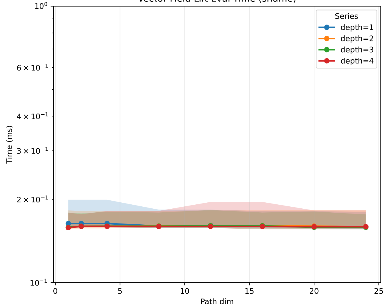
Vector Field Lift Eval Time (shuffle)
