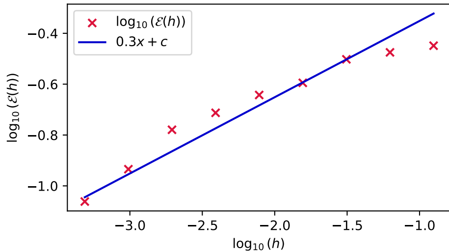
\mathcal{E}(h) for CF-EES _{\mathcal{R}}(2, 7)
