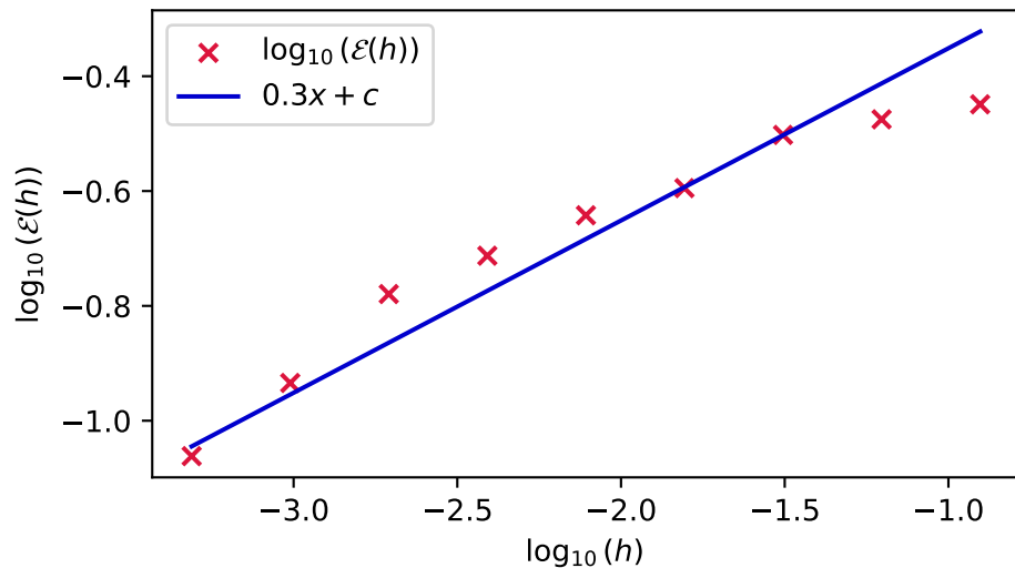
\mathcal{E}(h) for CF-EES _{\mathcal{R}}(2, 5)
