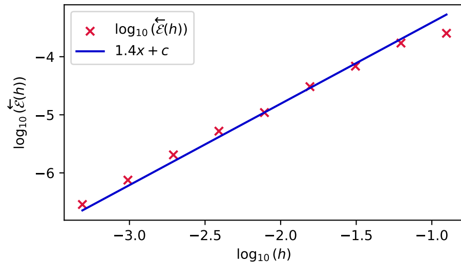
\overleftarrow{\mathcal{E}}(h) for CF-EES _{\mathcal{R}}(2, 5)
