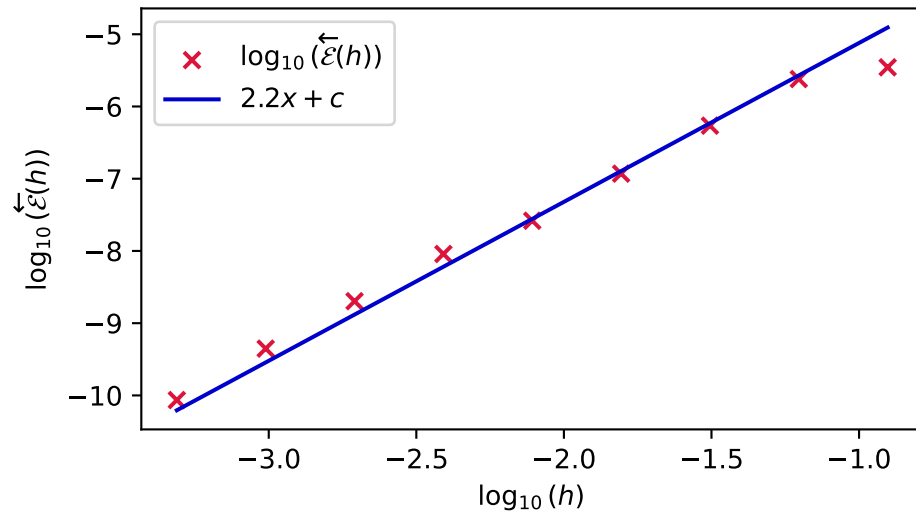
\overleftarrow{\mathcal{E}}(h) for CF-EES _{\mathcal{R}}(2, 7)
