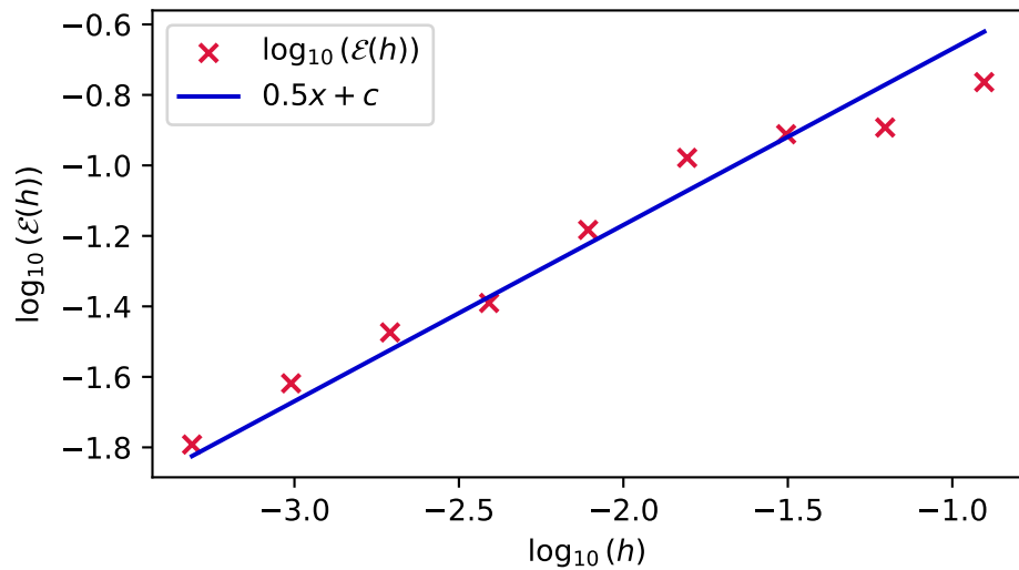
\mathcal{E}(h) for CF-EES _{\mathcal{R}}(2, 7)
