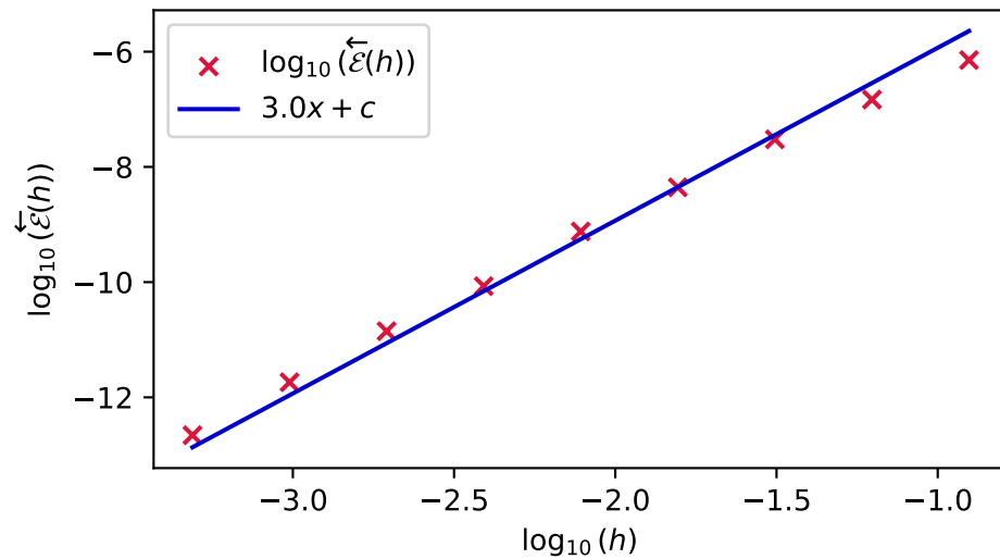
\overleftarrow{\mathcal{E}}(h) for CF-EES _{\mathcal{R}}(2, 7)
