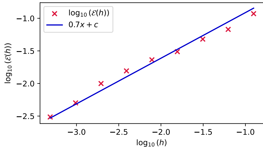
\mathcal{E}(h) for CF-EES _{\mathcal{R}}(2, 5)
