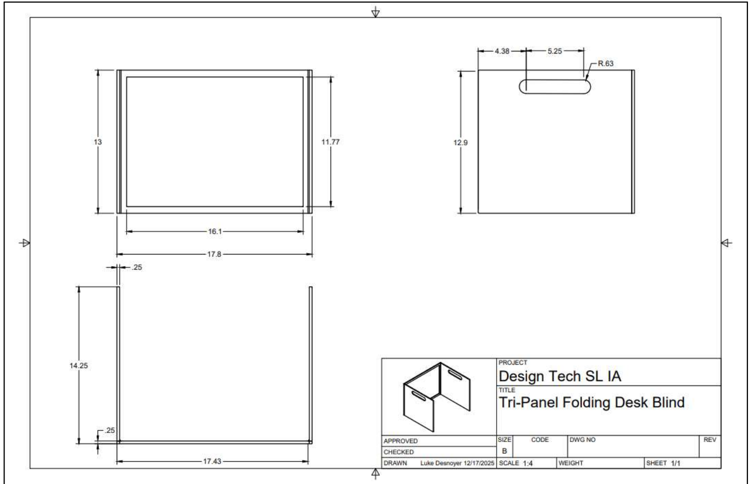
Figure 6. Design Sheet
