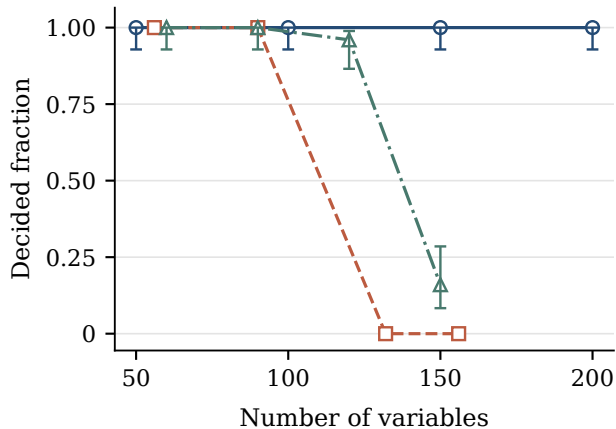
(b) A2: 10^6 conflict budget
