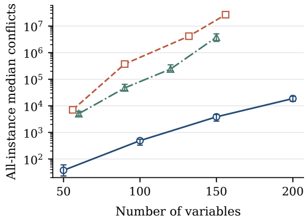
(a) A1: R1-certified, 3 \times 10^8 budget
