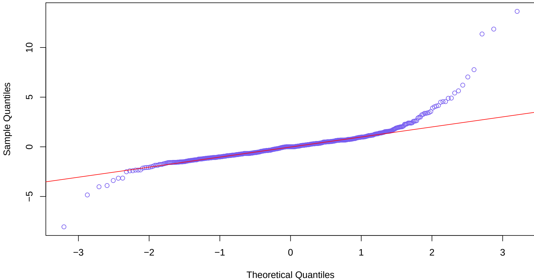
Normal QQ-Plot of MAD-Transformed data
