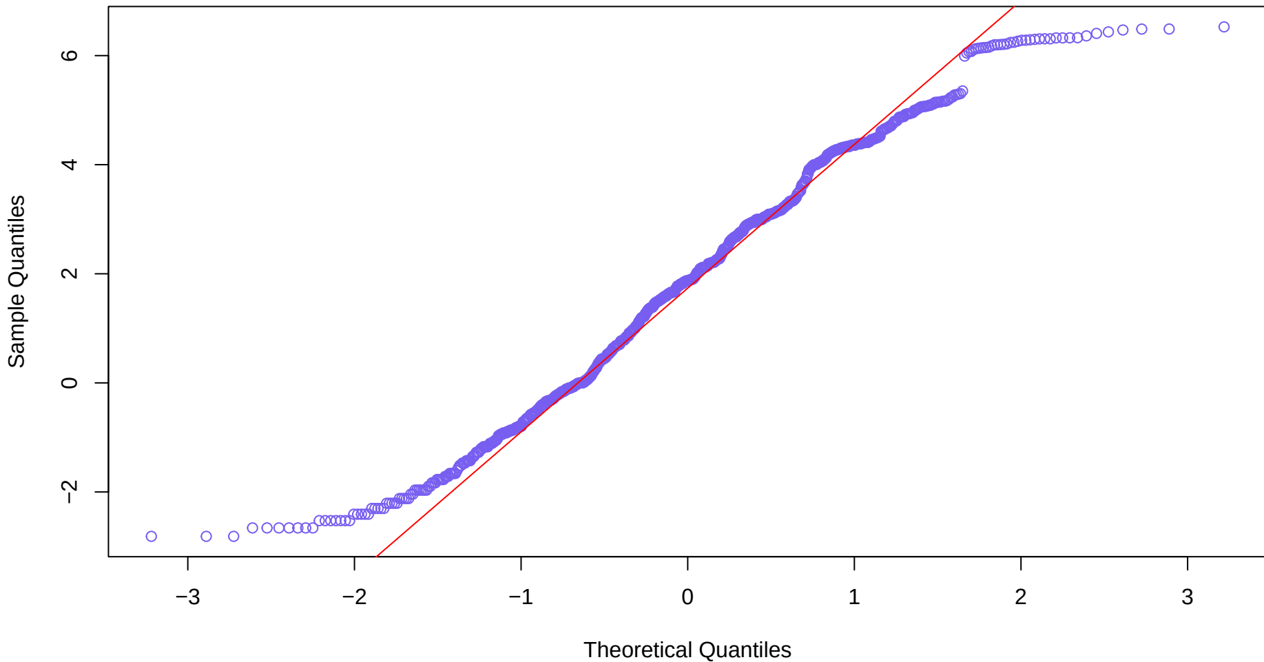
Normal QQ- Plot of the log-transformed data (all elements)
