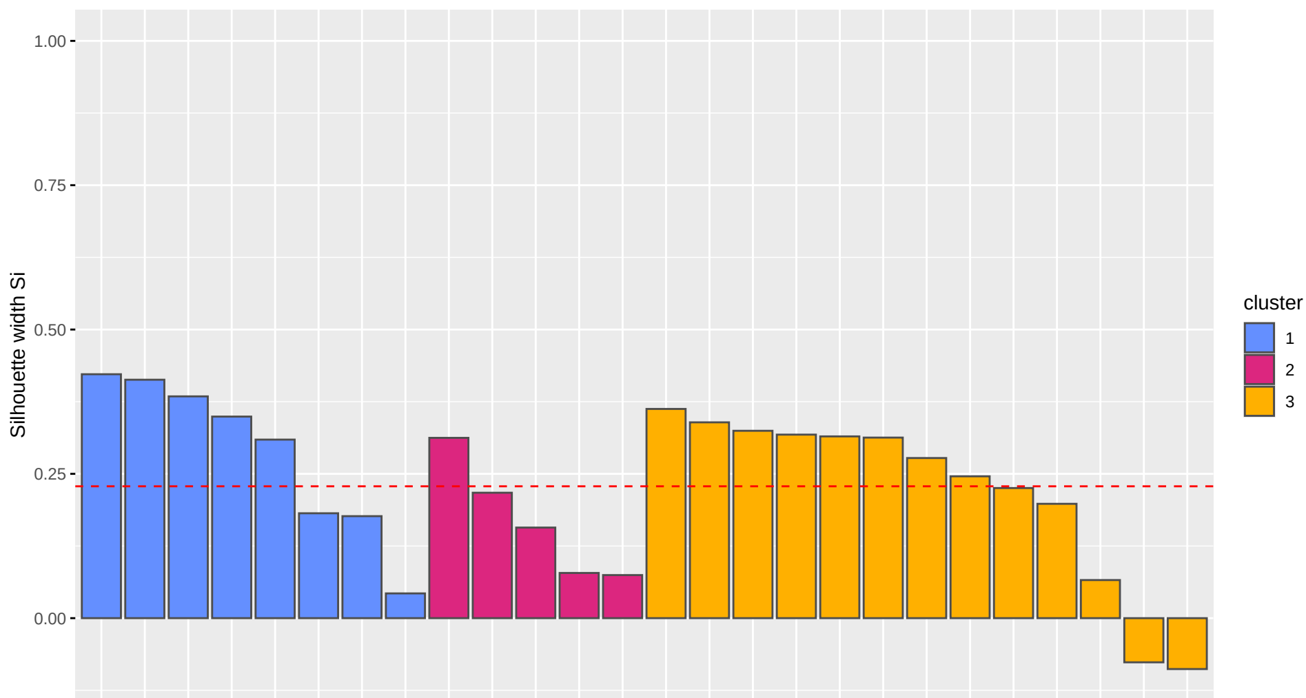
Clusters silhouette plot Average silhouette width: 0.23
