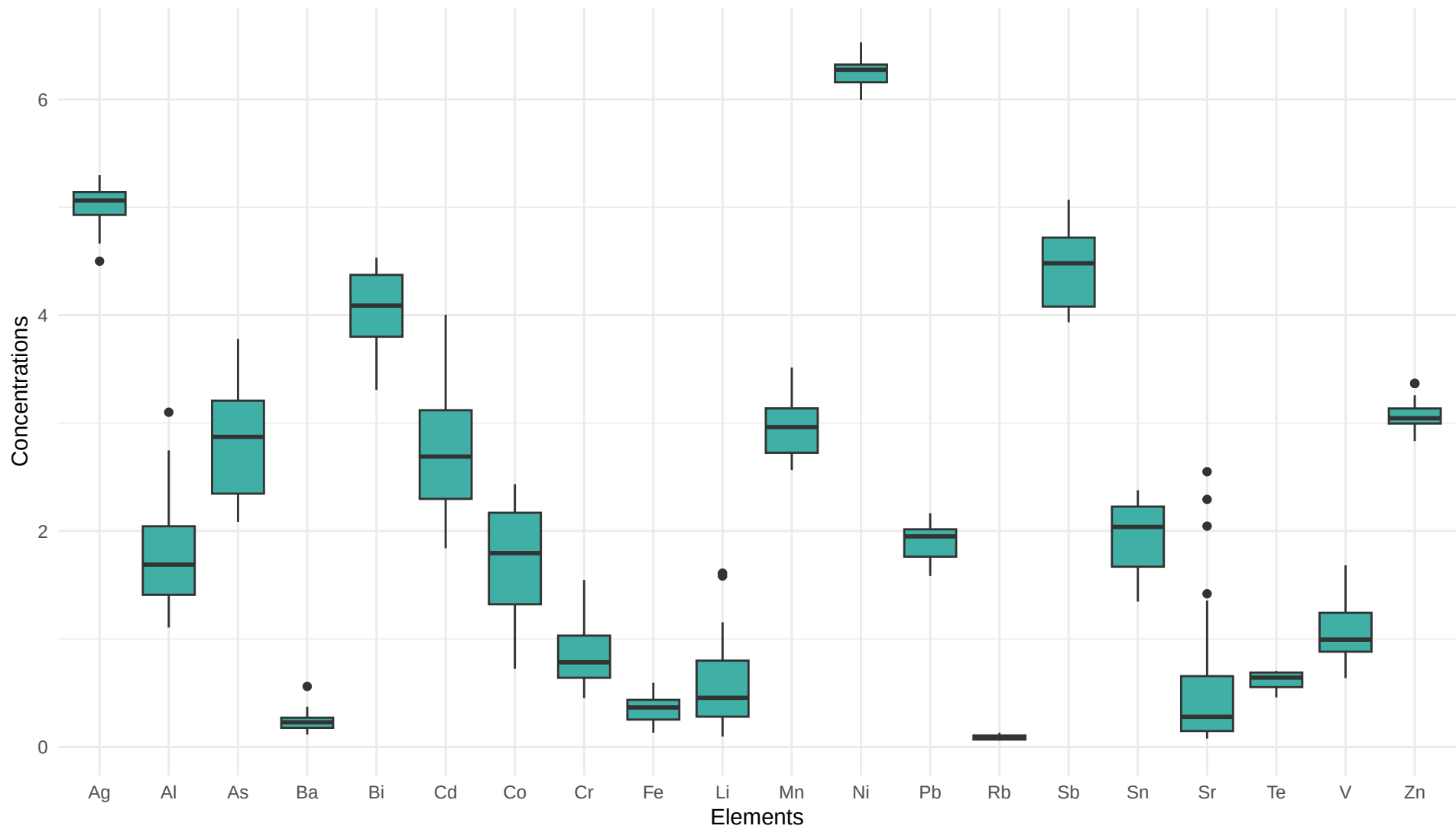
Boxplot of MAD Transformation With Outliers Removed
