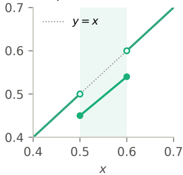
HeLU, zoom on the notch
