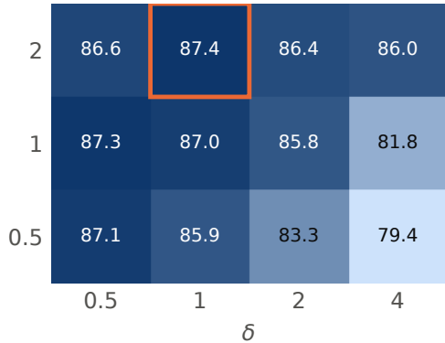
Fashion-MNIST validation acc. (%)
