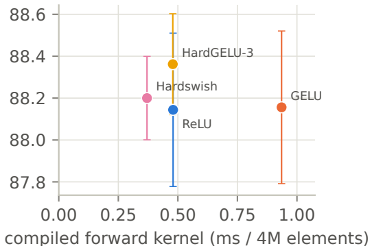
Cost vs. accuracy
