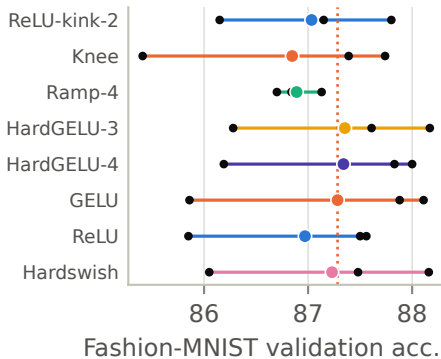
Screen (3 ep., 3 seeds)
